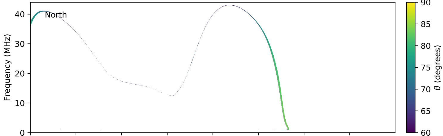
expres_earth_jupiter_io_jrm09_lossc-wid1deg_3kev_20150131_v01.cdf
