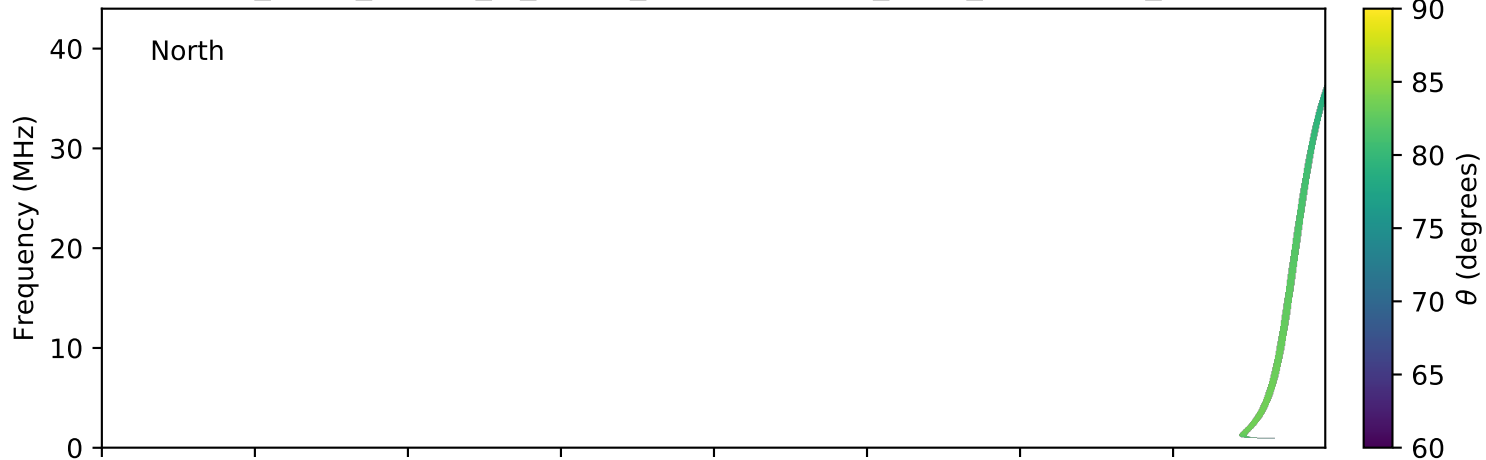
expres_earth_jupiter_io_jrm09_lossc-wid1deg_3kev_20150130_v01.cdf
