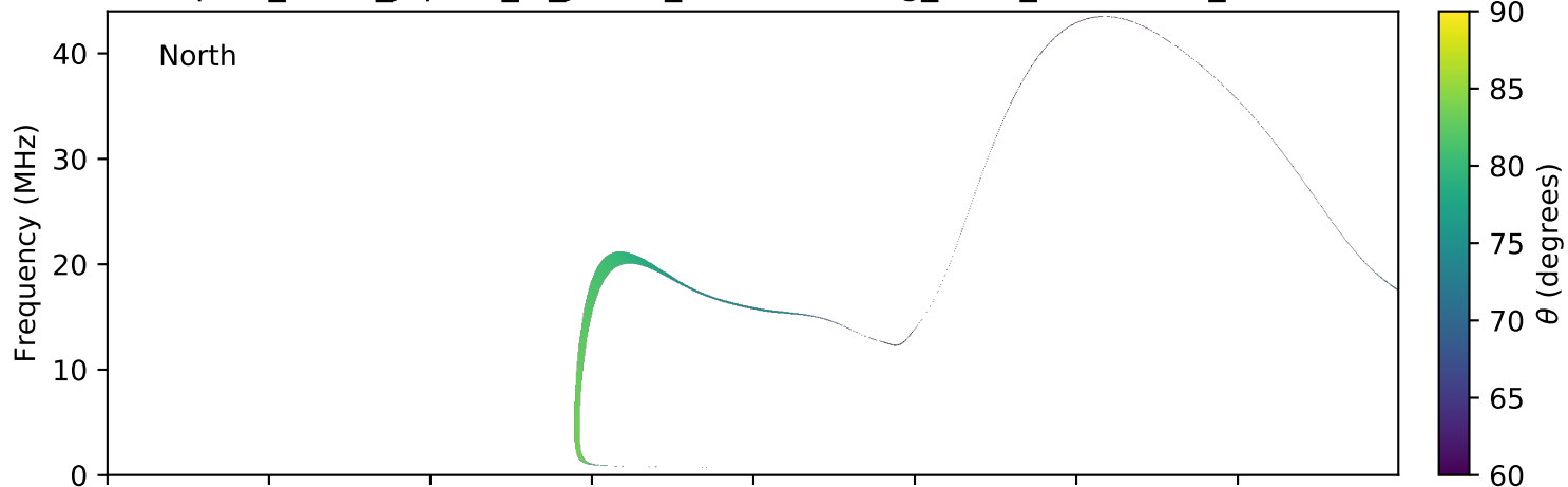
expres_earth_jupiter_io_jrm09_lossc-wid1deg_3kev_20150127_v01.cdf
