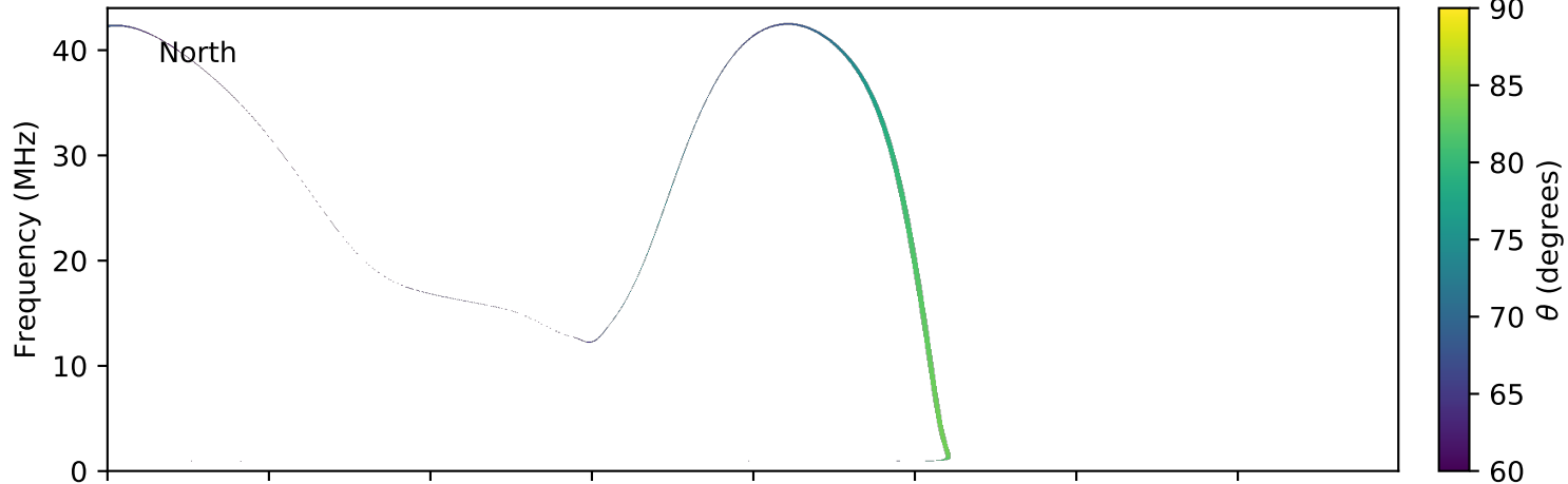
expres_earth_jupiter_io_jrm09_lossc-wid1deg_3kev_20150124_v01.cdf
