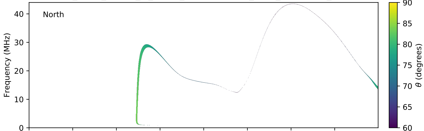
expres_earth_jupiter_io_jrm09_lossc-wid1deg_3kev_20150120_v01.cdf
