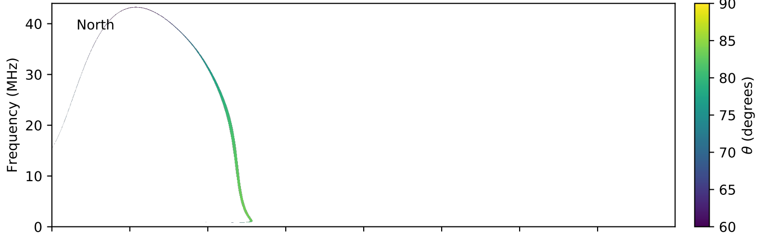
expres_earth_jupiter_io_jrm09_lossc-wid1deg_3kev_20150119_v01.cdf
