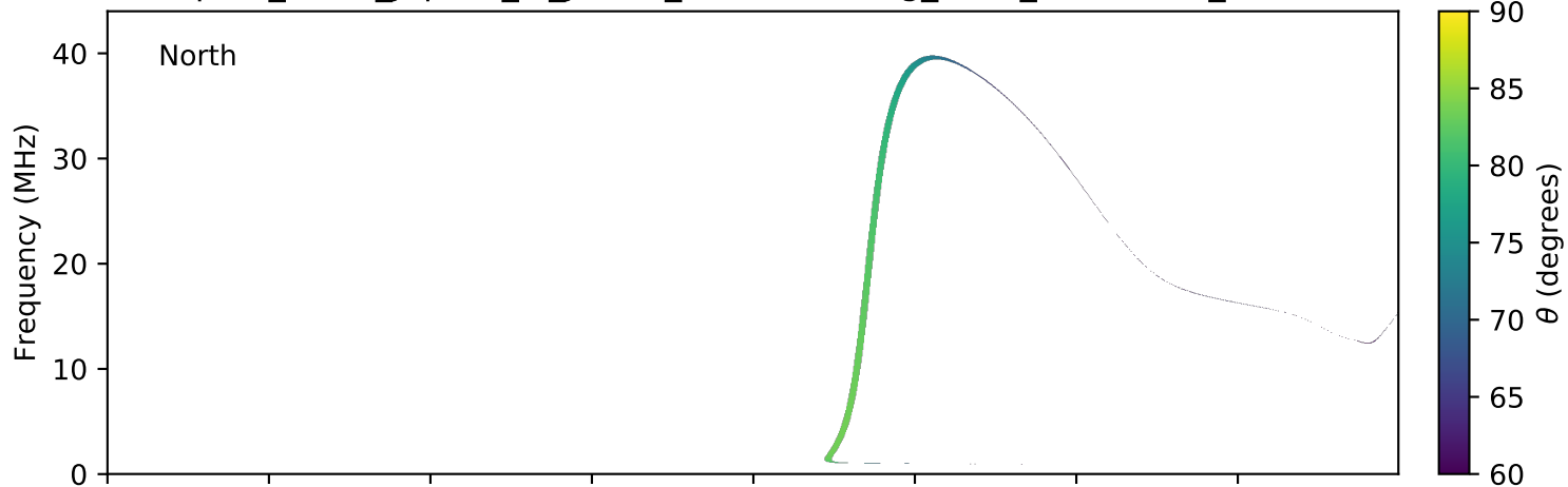
expres_earth_jupiter_io_jrm09_lossc-wid1deg_3kev_20150118_v01.cdf
