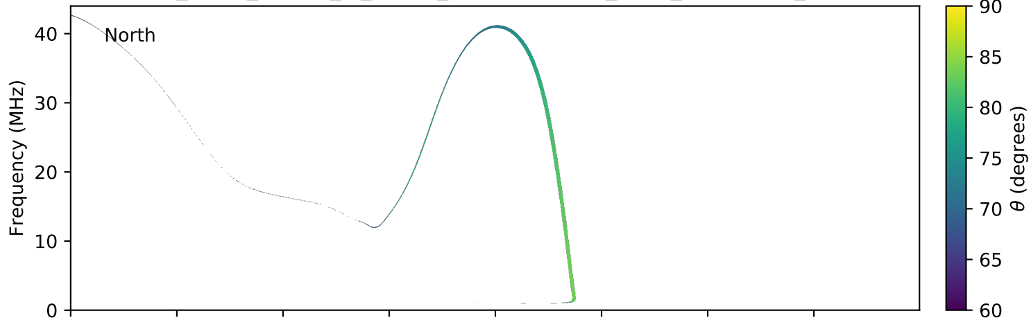
expres_earth_jupiter_io_jrm09_lossc-wid1deg_3kev_20150117_v01.cdf
