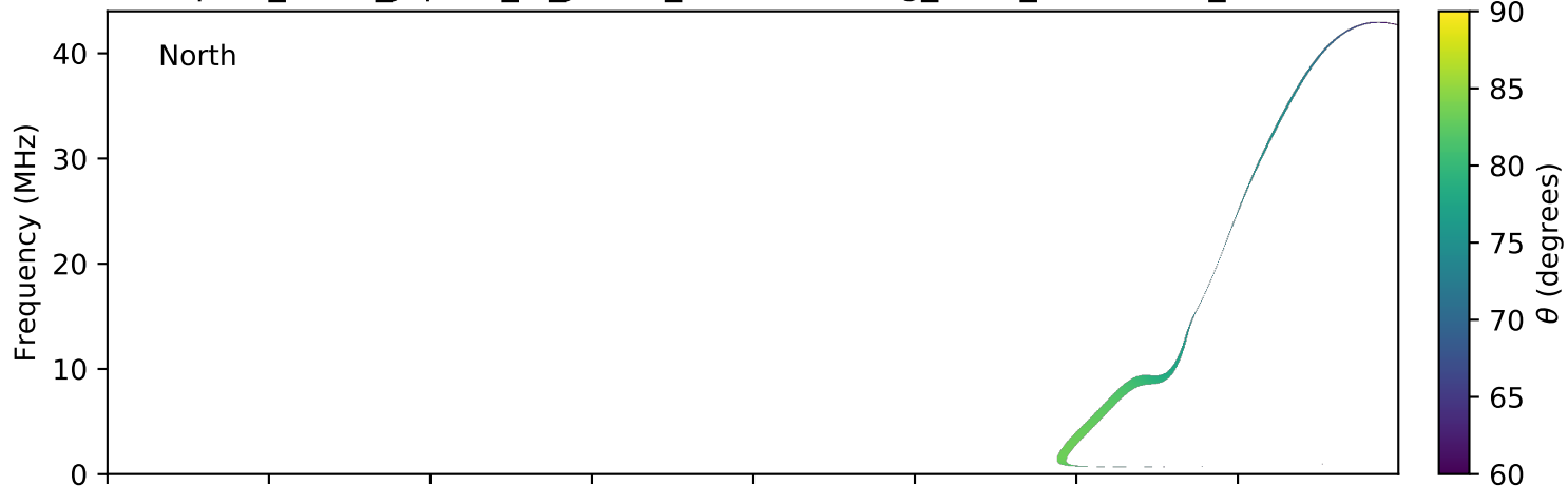
expres_earth_jupiter_io_jrm09_lossc-wid1deg_3kev_20150116_v01.cdf
