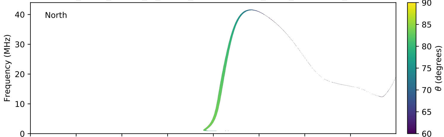
expres_earth_jupiter_io_jrm09_lossc-wid1deg_3kev_20150111_v01.cdf
