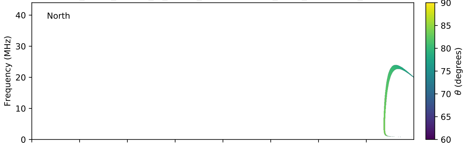
expres_earth_jupiter_io_jrm09_lossc-wid1deg_3kev_20150107_v01.cdf
