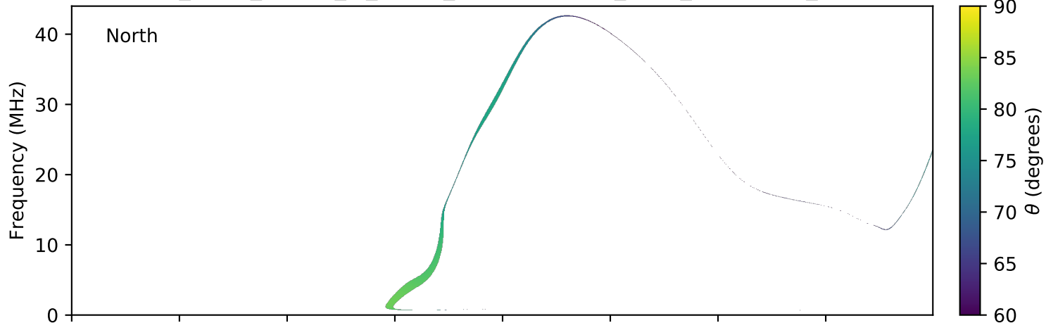
expres_earth_jupiter_io_jrm09_lossc-wid1deg_3kev_20150104_v01.cdf
