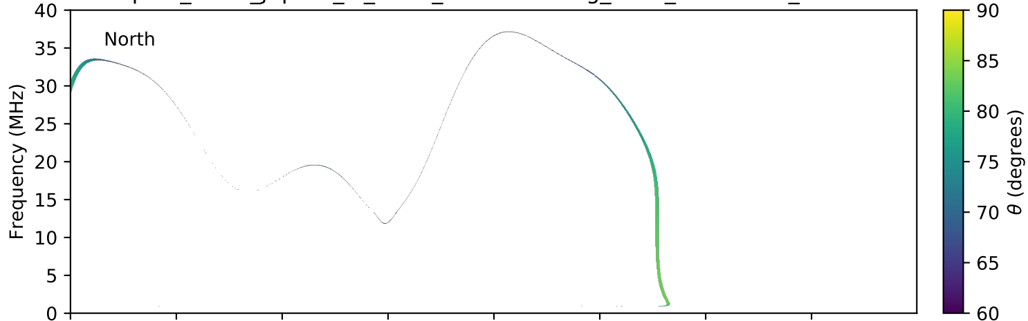
expres_earth_jupiter_io_isaac_lossc-wid1deg_3kev_20150131_v01.cdf
