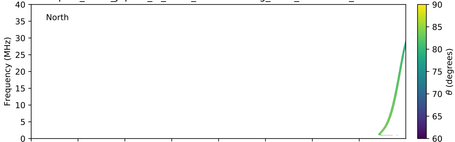
expres_earth_jupiter_io_isaac_lossc-wid1deg_3kev_20150130_v01.cdf
