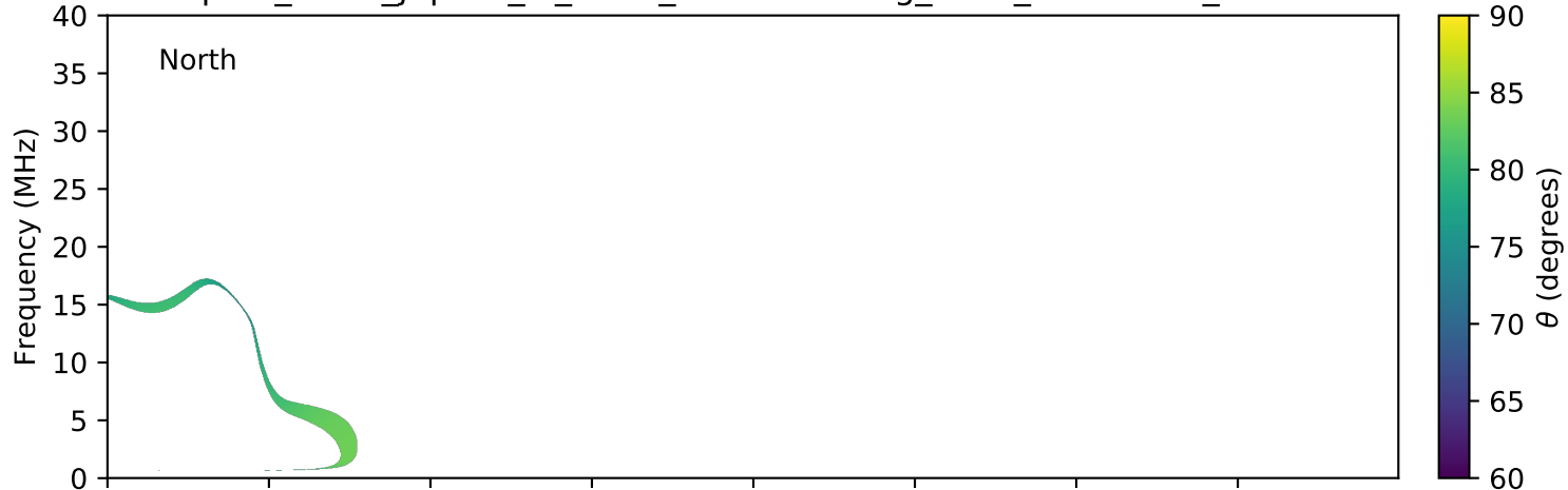
expres_earth_jupiter_io_isaac_lossc-wid1deg_3kev_20150128_v01.cdf
