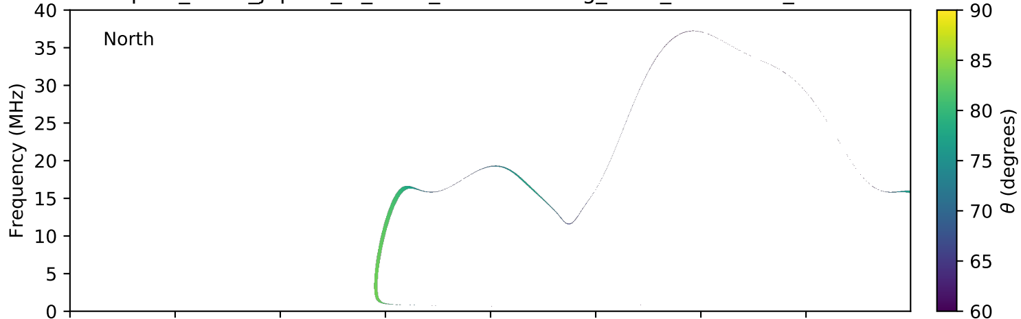
expres_earth_jupiter_io_isaac_lossc-wid1deg_3kev_20150127_v01.cdf
