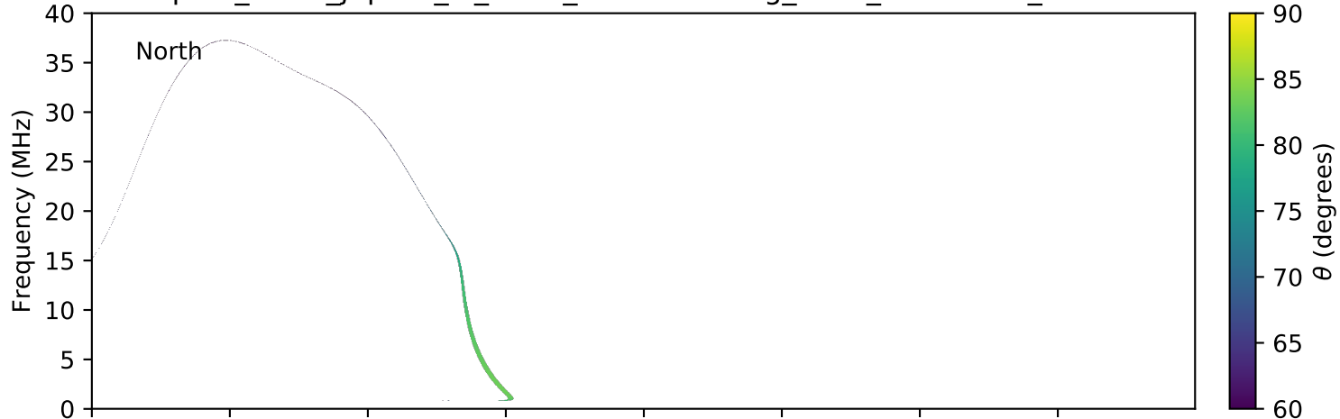
expres_earth_jupiter_io_isaac_lossc-wid1deg_3kev_20150126_v01.cdf
