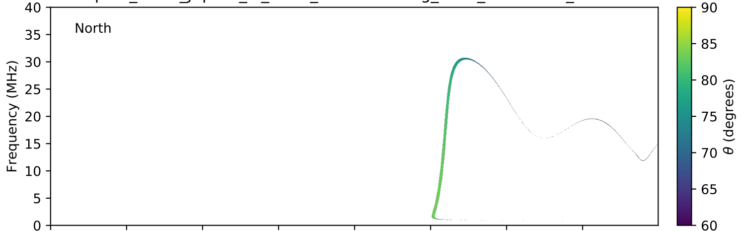
expres_earth_jupiter_io_isaac_lossc-wid1deg_3kev_20150125_v01.cdf
