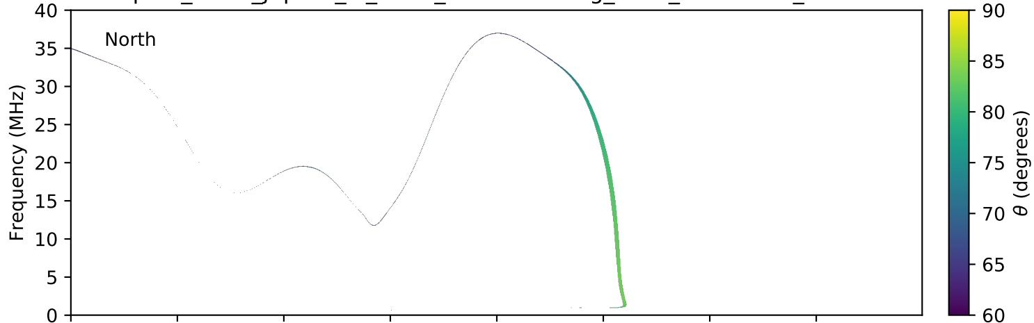
expres_earth_jupiter_io_isaac_lossc-wid1deg_3kev_20150124_v01.cdf
