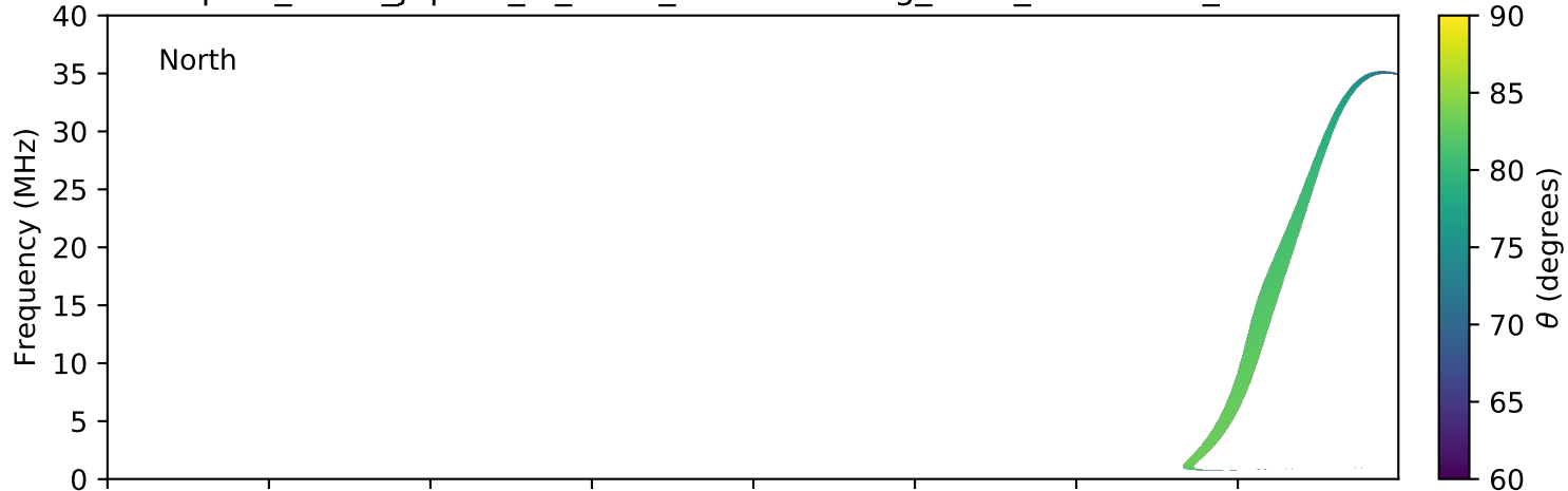
expres_earth_jupiter_io_isaac_lossc-wid1deg_3kev_20150123_v01.cdf
