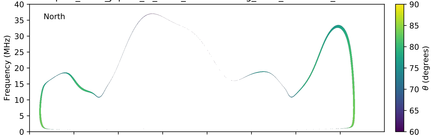
expres_earth_jupiter_io_isaac_lossc-wid1deg_3kev_20150122_v01.cdf
