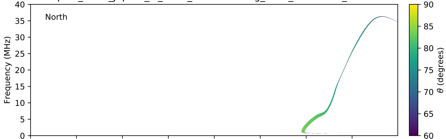
expres_earth_jupiter_io_isaac_lossc-wid1deg_3kev_20150116_v01.cdf
