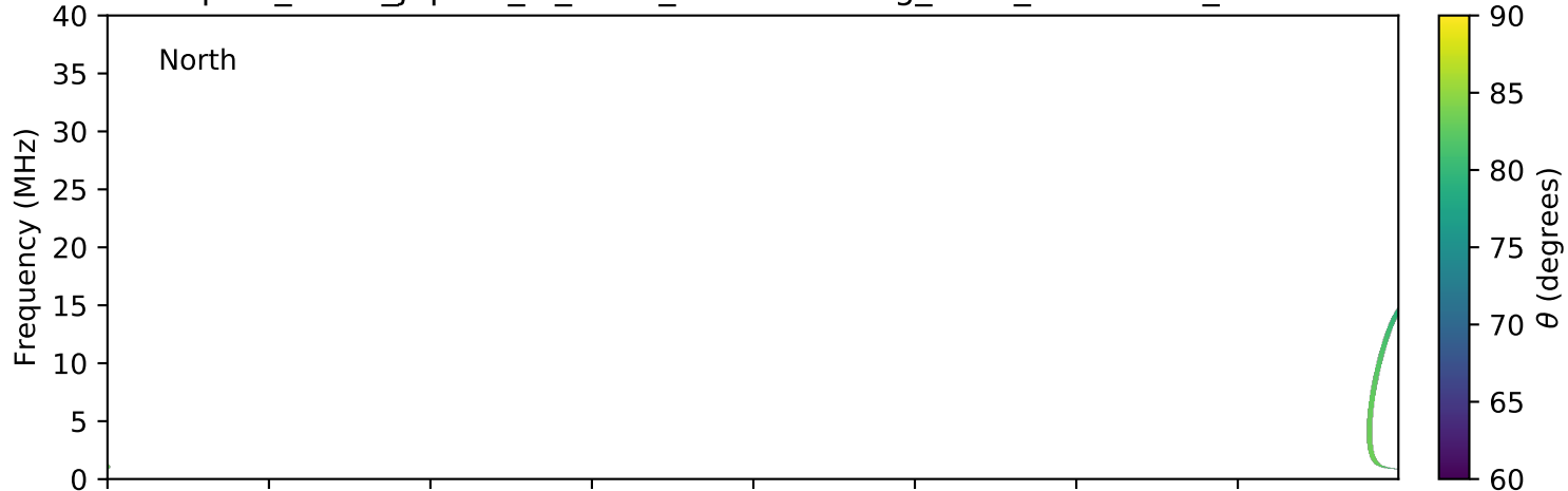
expres_earth_jupiter_io_isaac_lossc-wid1deg_3kev_20150114_v01.cdf
