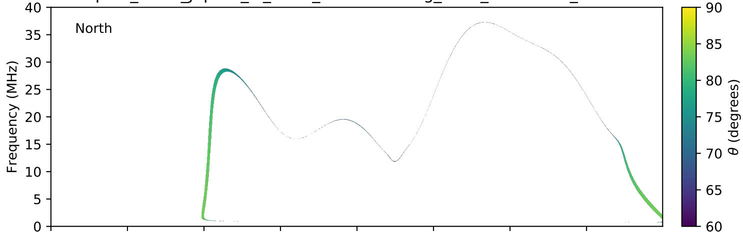
expres_earth_jupiter_io_isaac_lossc-wid1deg_3kev_20150113_v01.cdf
