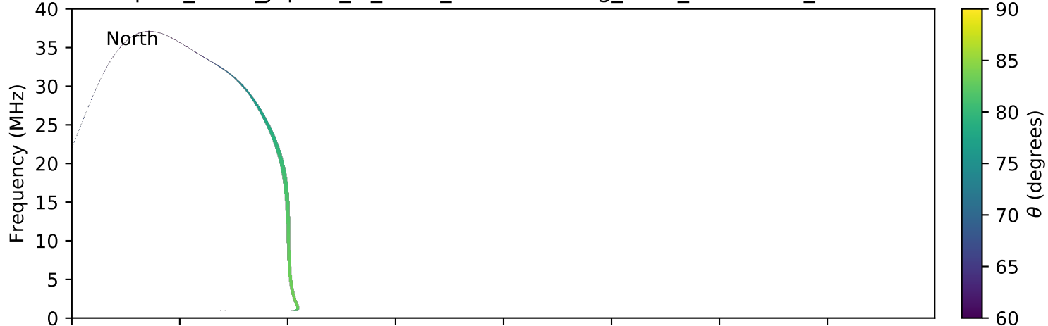
expres_earth_jupiter_io_isaac_lossc-wid1deg_3kev_20150112_v01.cdf
