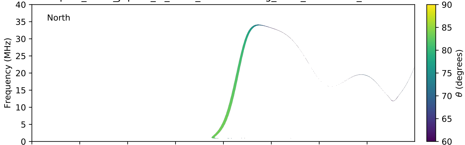
expres_earth_jupiter_io_isaac_lossc-wid1deg_3kev_20150111_v01.cdf
