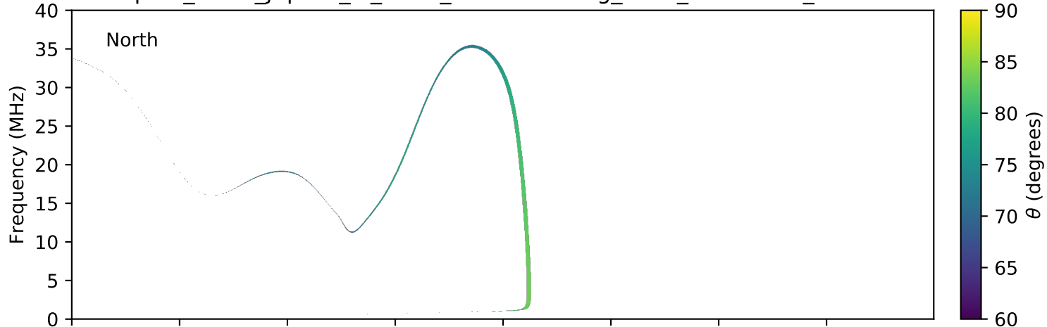
expres_earth_jupiter_io_isaac_lossc-wid1deg_3kev_20150110_v01.cdf
