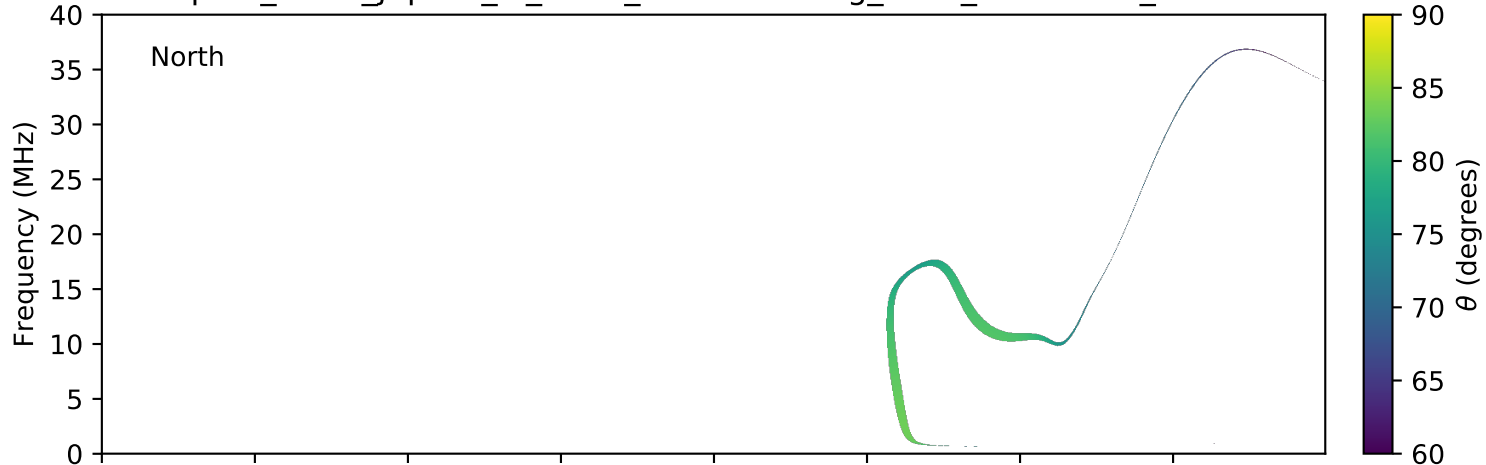
expres_earth_jupiter_io_isaac_lossc-wid1deg_3kev_20150109_v01.cdf
