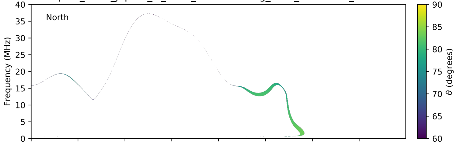
expres_earth_jupiter_io_isaac_lossc-wid1deg_3kev_20150108_v01.cdf
