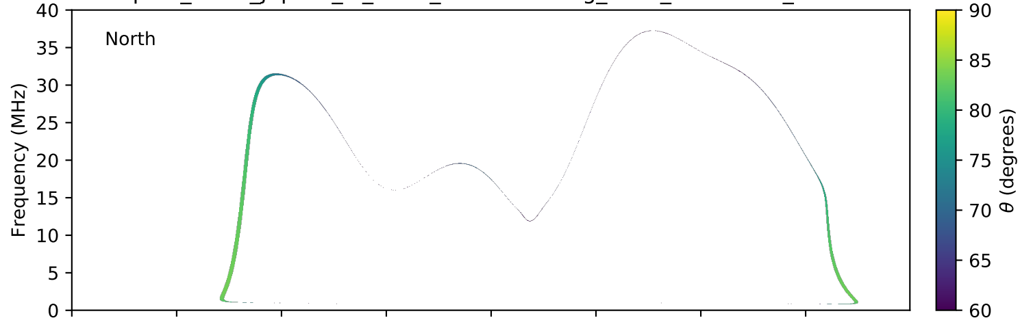
expres_earth_jupiter_io_isaac_lossc-wid1deg_3kev_20150106_v01.cdf
