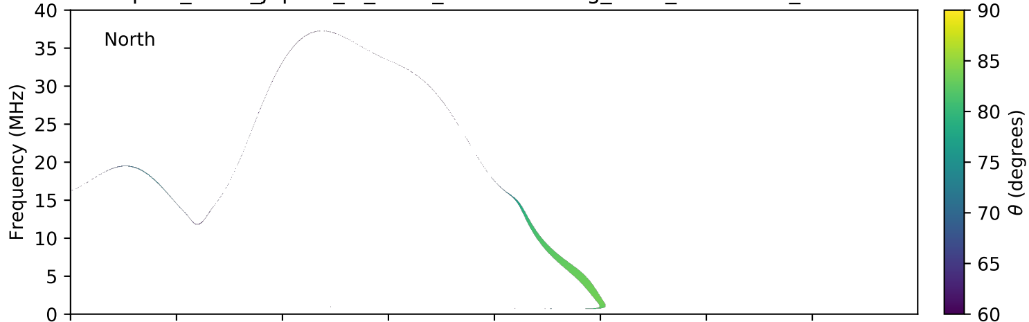
expres_earth_jupiter_io_isaac_lossc-wid1deg_3kev_20150101_v01.cdf
