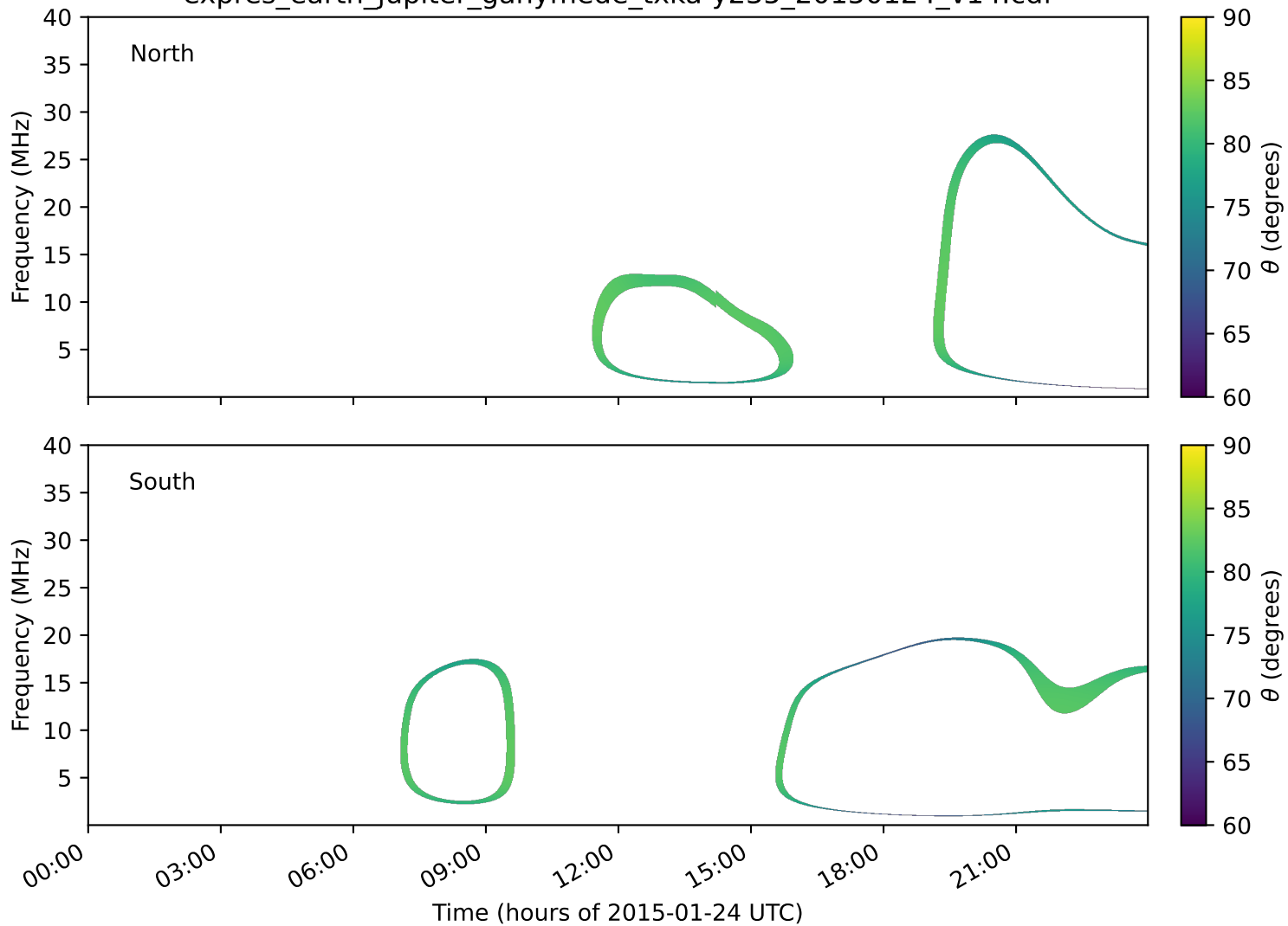
expres_earth_jupiter_ganymede_txka-y235_20150124_v14.cdf
