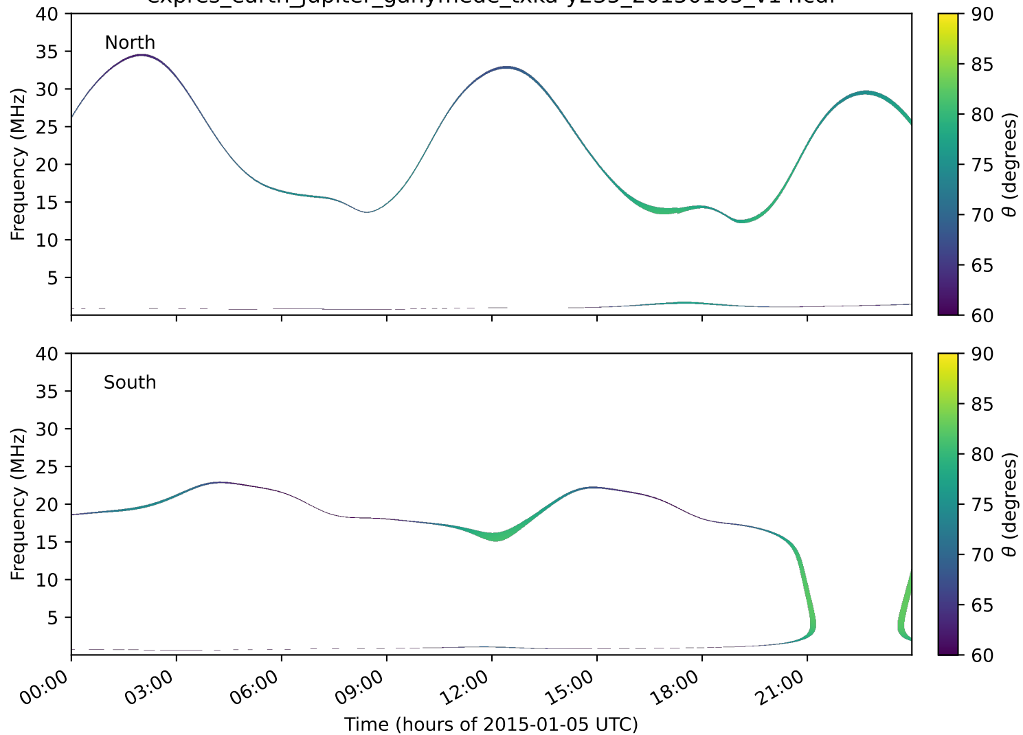
expres_earth_jupiter_ganymede_txka-y235_20150105_v14.cdf
