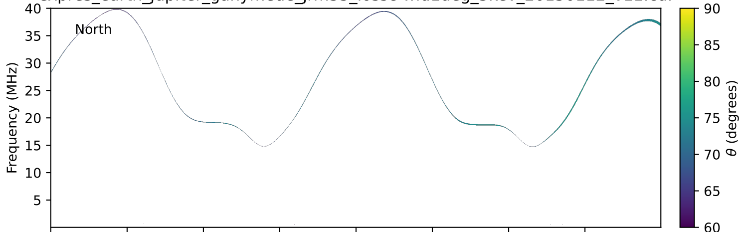
expres_earth_jupiter_ganymede_jrm33_lossc-wid1deg_3kev_20150112_v11.cdf
