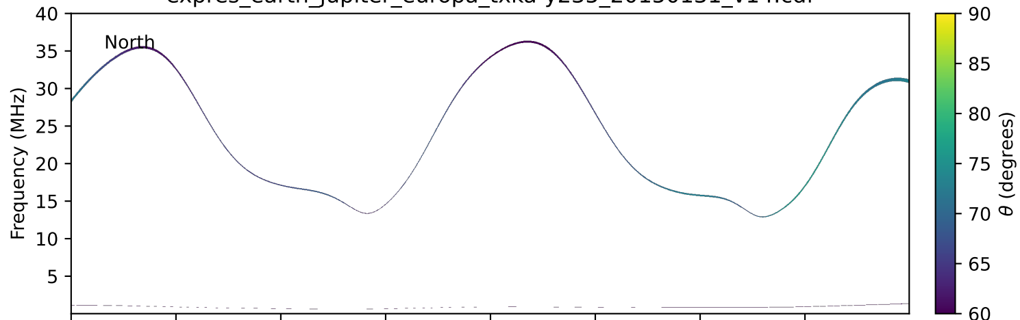
expres_earth_jupiter_europa_txka-y235_20150131_v14.cdf
