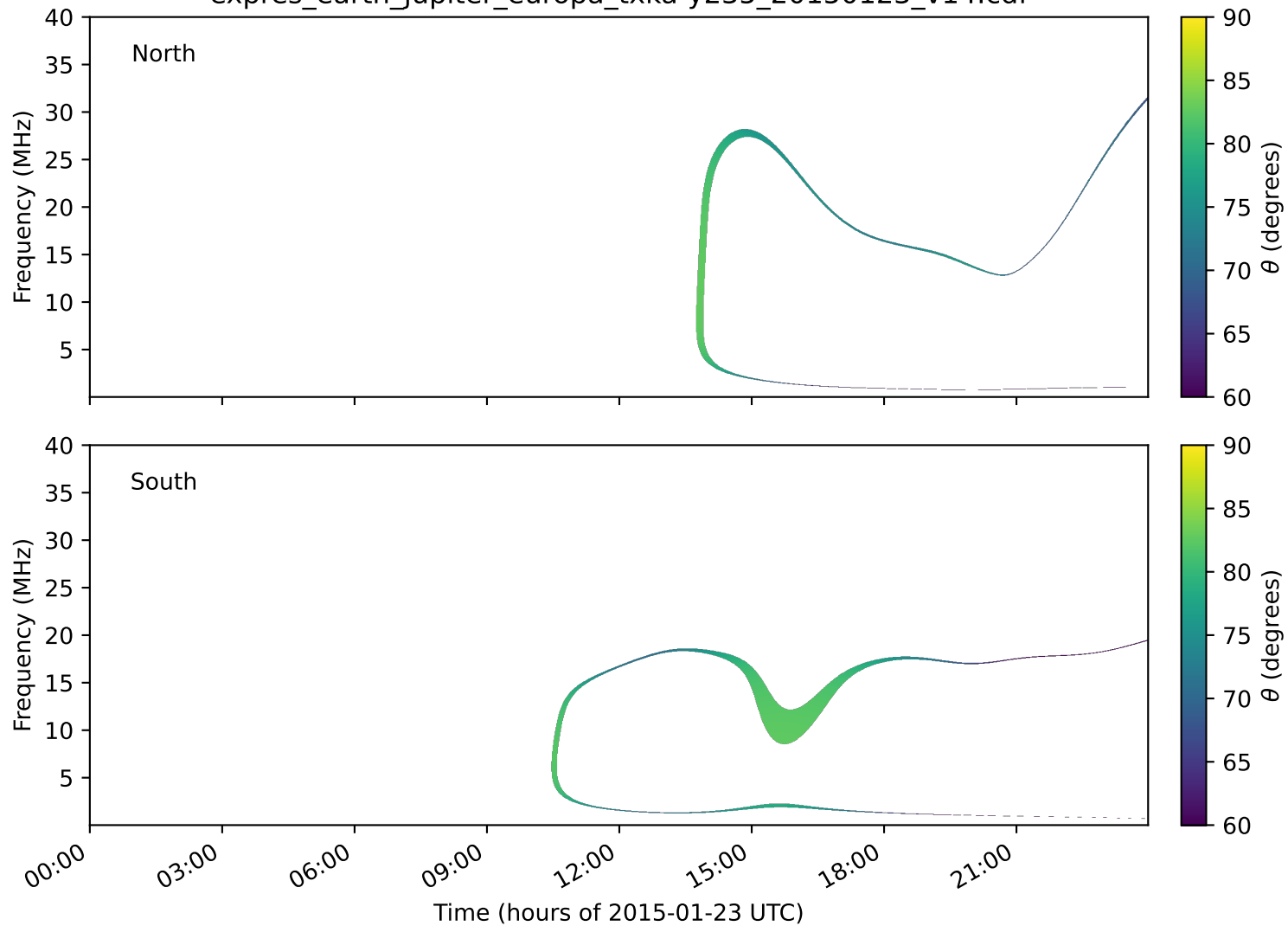
expres_earth_jupiter_europa_txka-y235_20150123_v14.cdf
