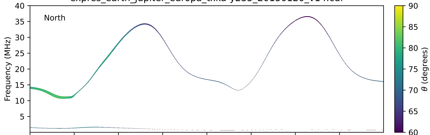
expres_earth_jupiter_europa_txka-y235_20150120_v14.cdf
