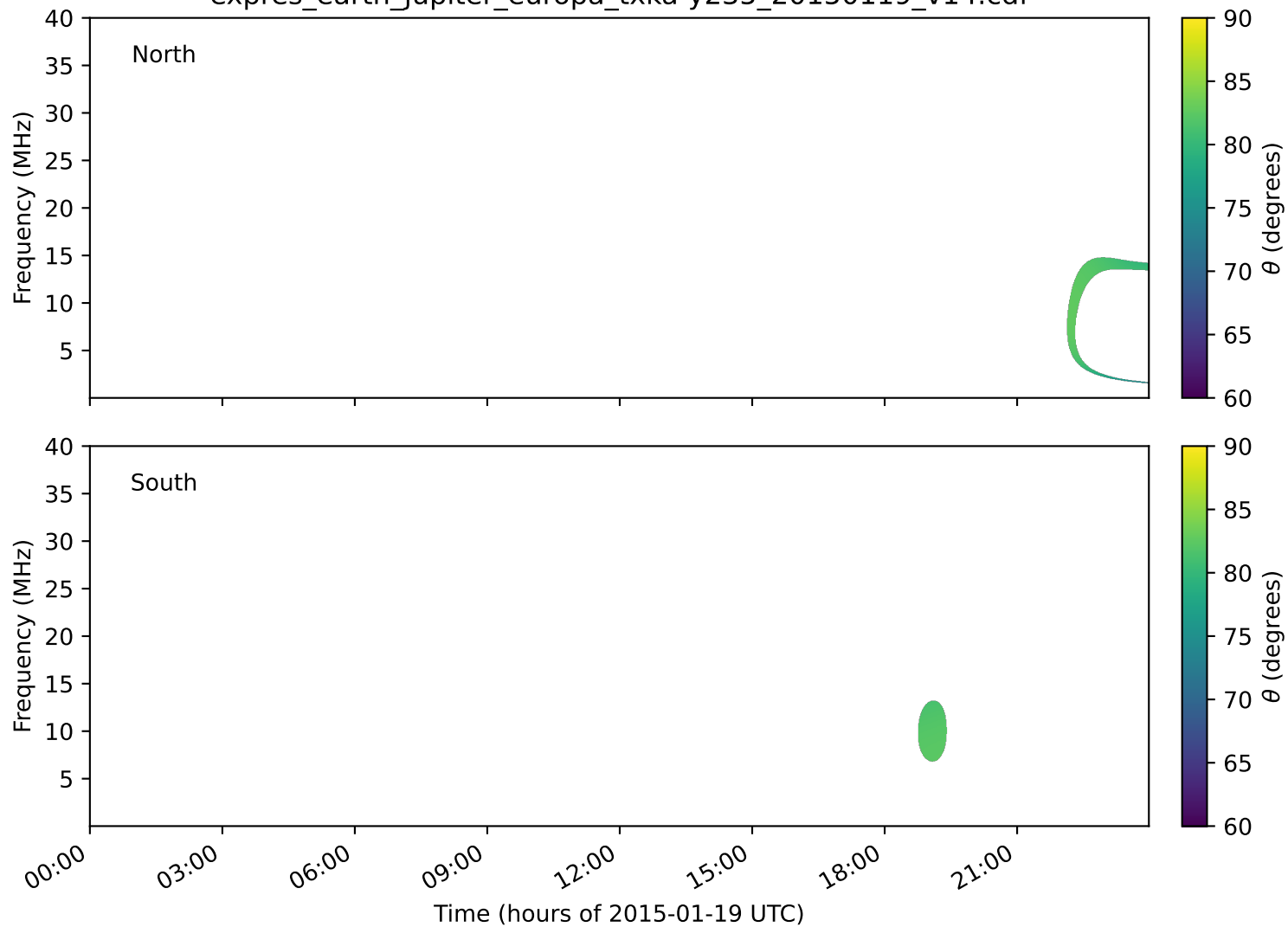
expres_earth_jupiter_europa_txka-y235_20150119_v14.cdf
