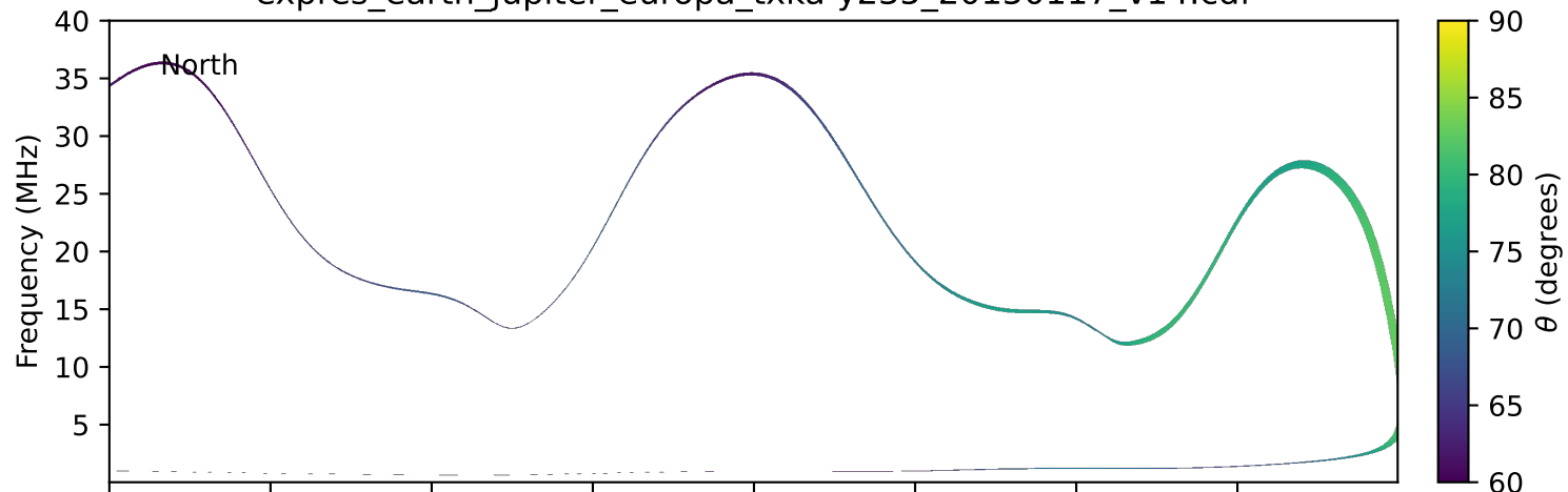
expres_earth_jupiter_europa_txka-y235_20150117_v14.cdf
