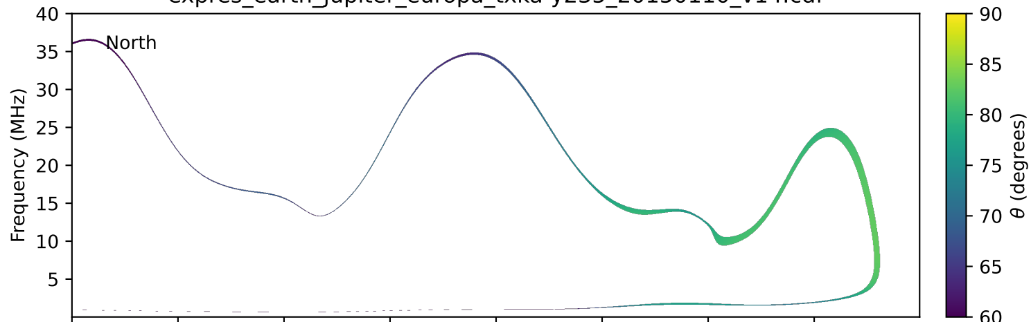
expres_earth_jupiter_europa_txka-y235_20150110_v14.cdf
