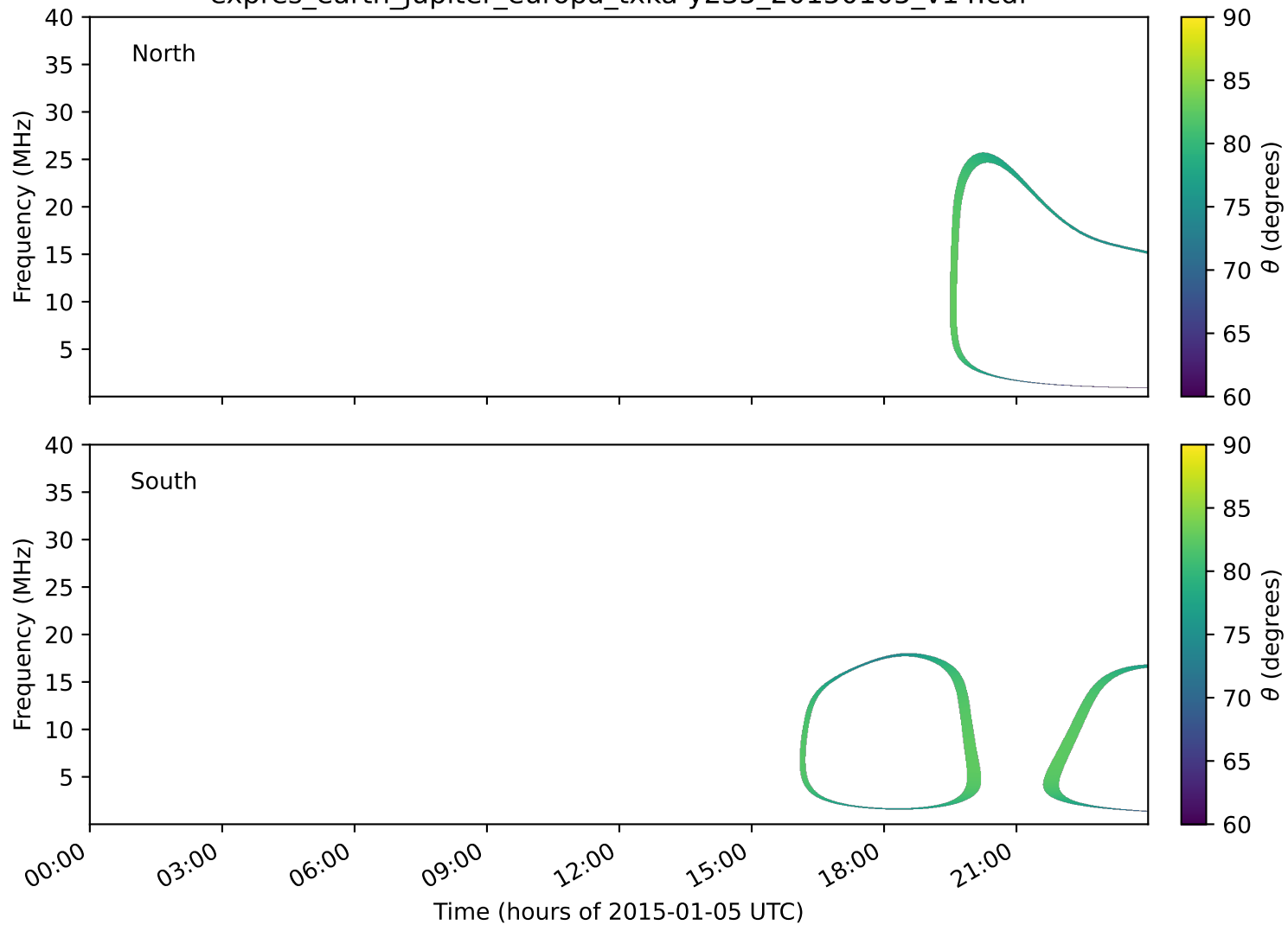
expres_earth_jupiter_europa_txka-y235_20150105_v14.cdf
