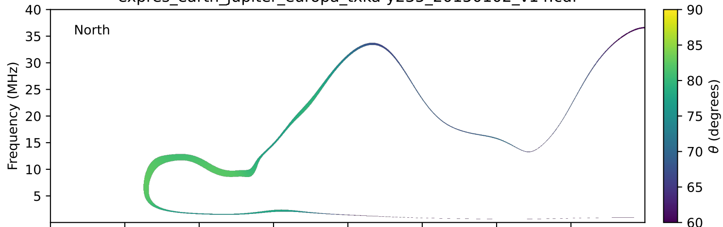
expres_earth_jupiter_europa_txka-y235_20150102_v14.cdf
