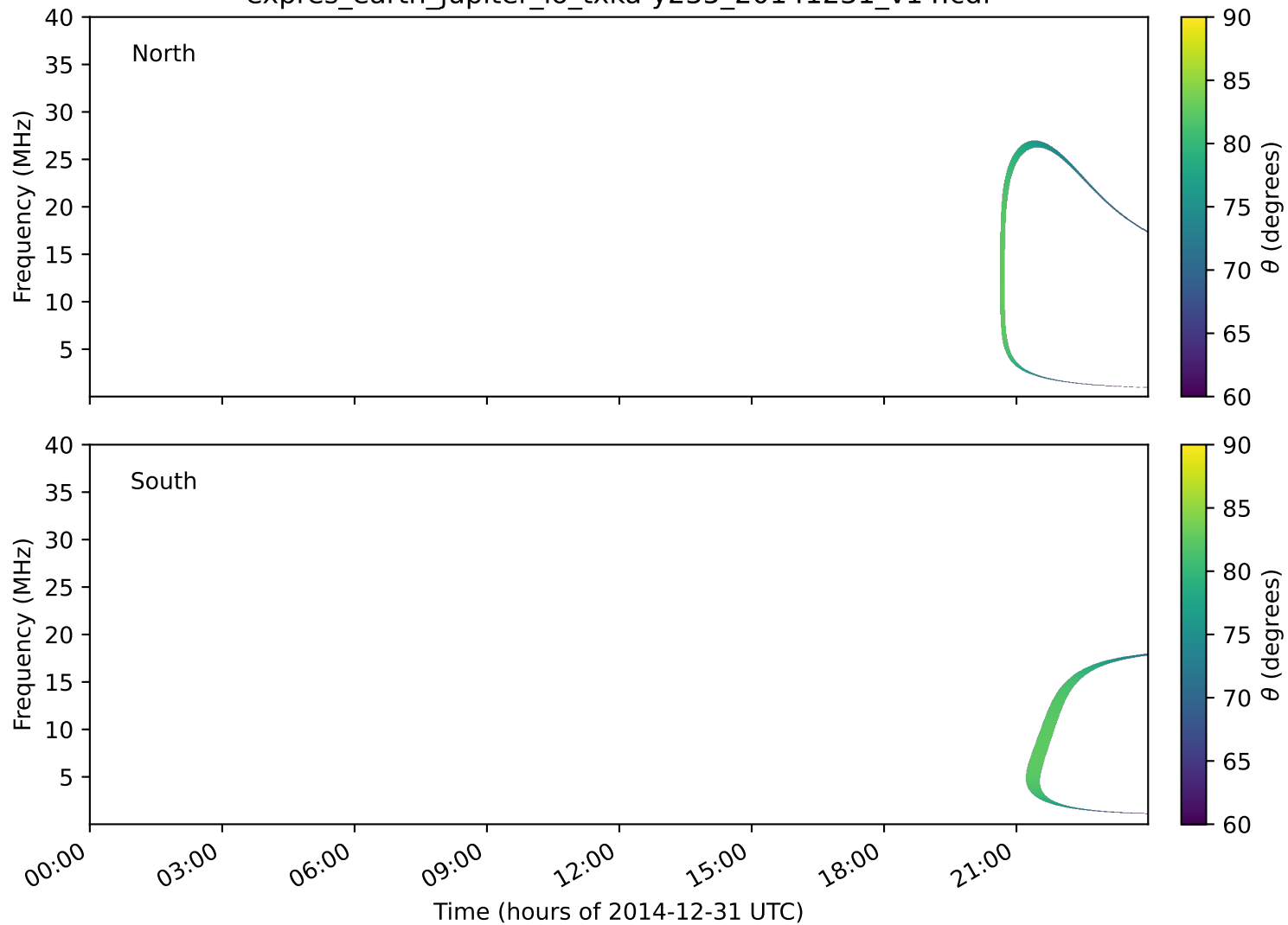
expres_earth_jupiter_io_txka-y235_20141231_v14.cdf
