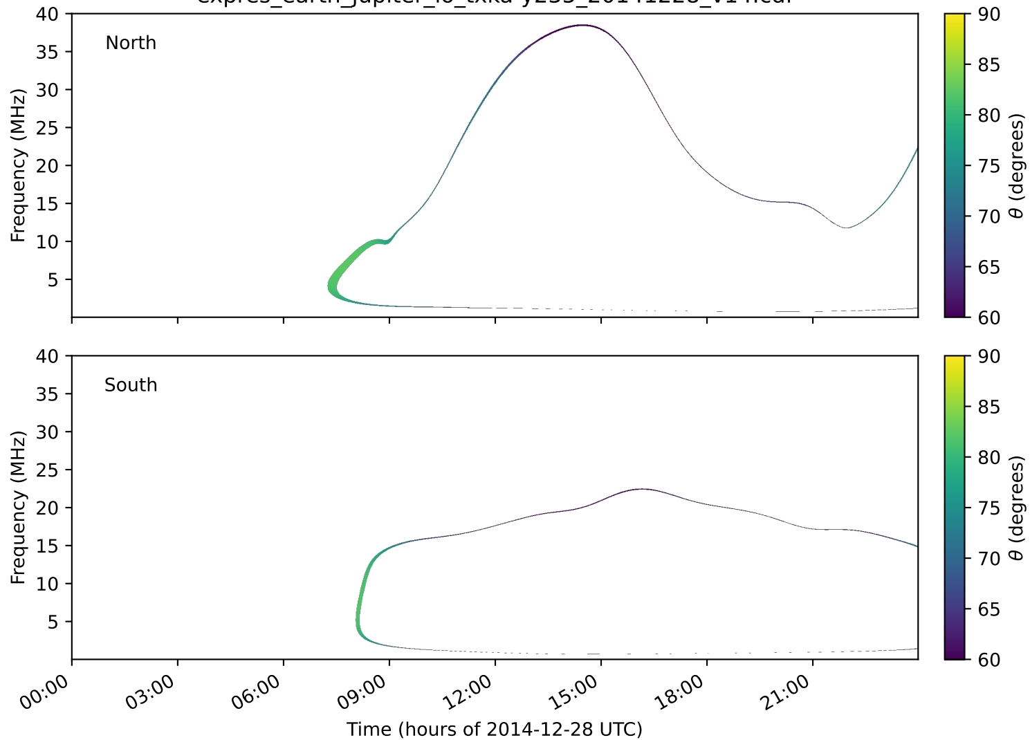
expres_earth_jupiter_io_txka-y235_20141228_v14.cdf
