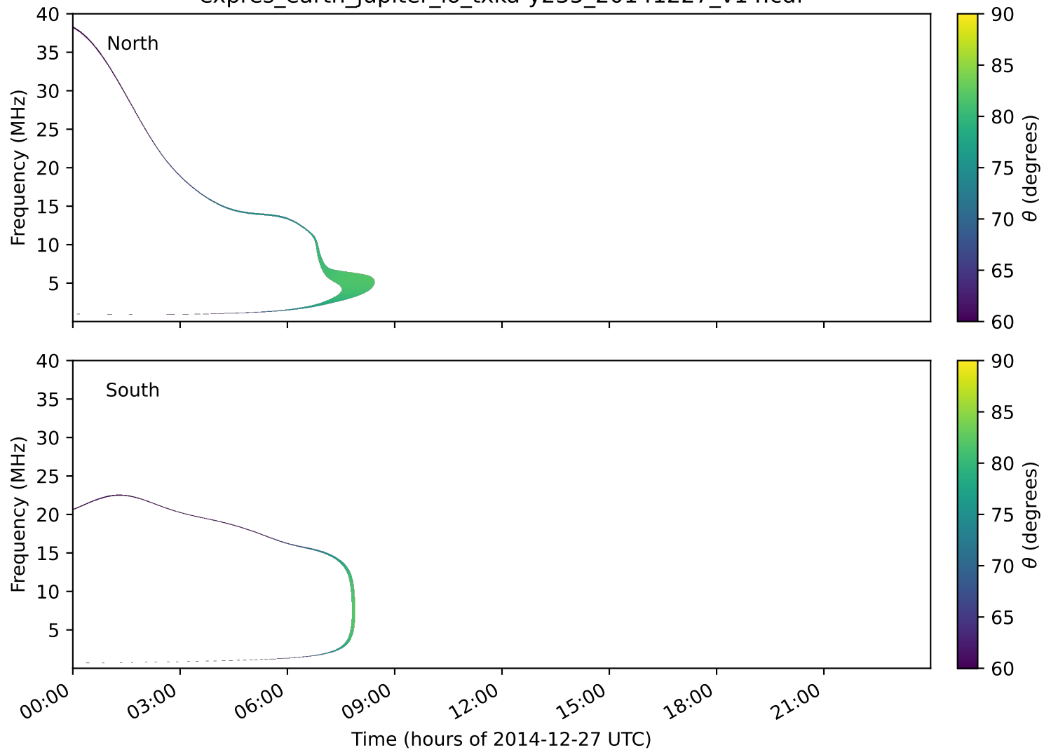
expres_earth_jupiter_io_txka-y235_20141227_v14.cdf
