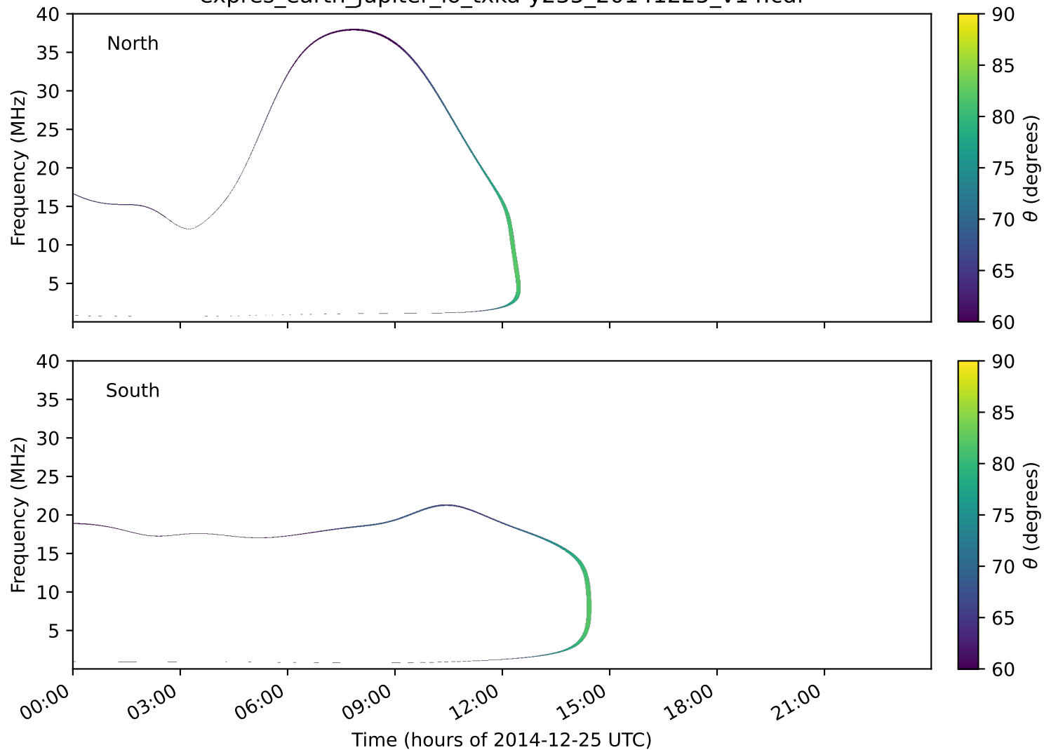
expres_earth_jupiter_io_txka-y235_20141225_v14.cdf
