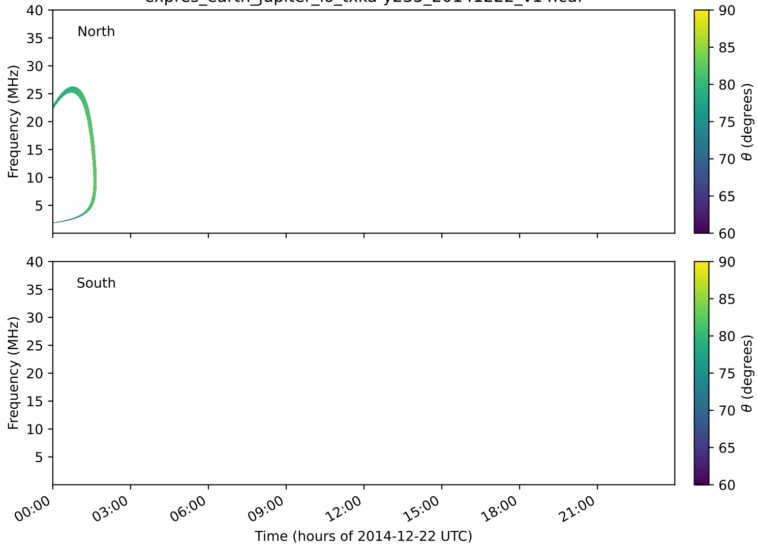
expres_earth_jupiter_io_txka-y235_20141222_v14.cdf
