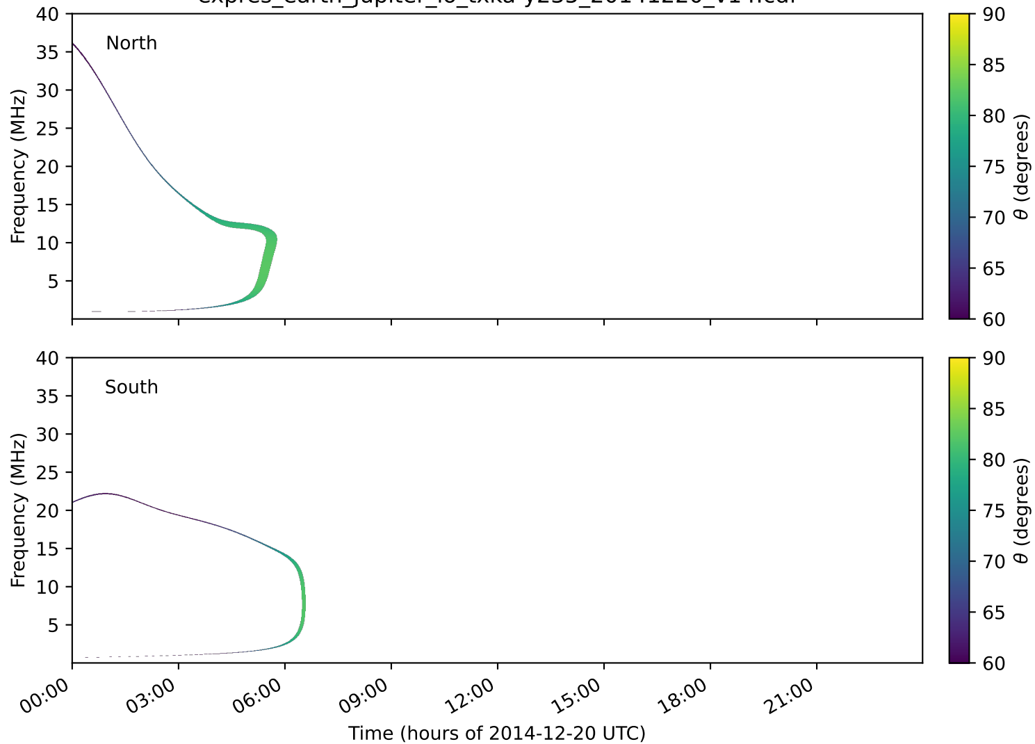
expres_earth_jupiter_io_txka-y235_20141220_v14.cdf
