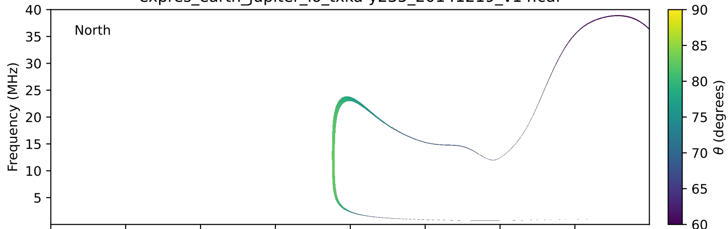
expres_earth_jupiter_io_txka-y235_20141219_v14.cdf
