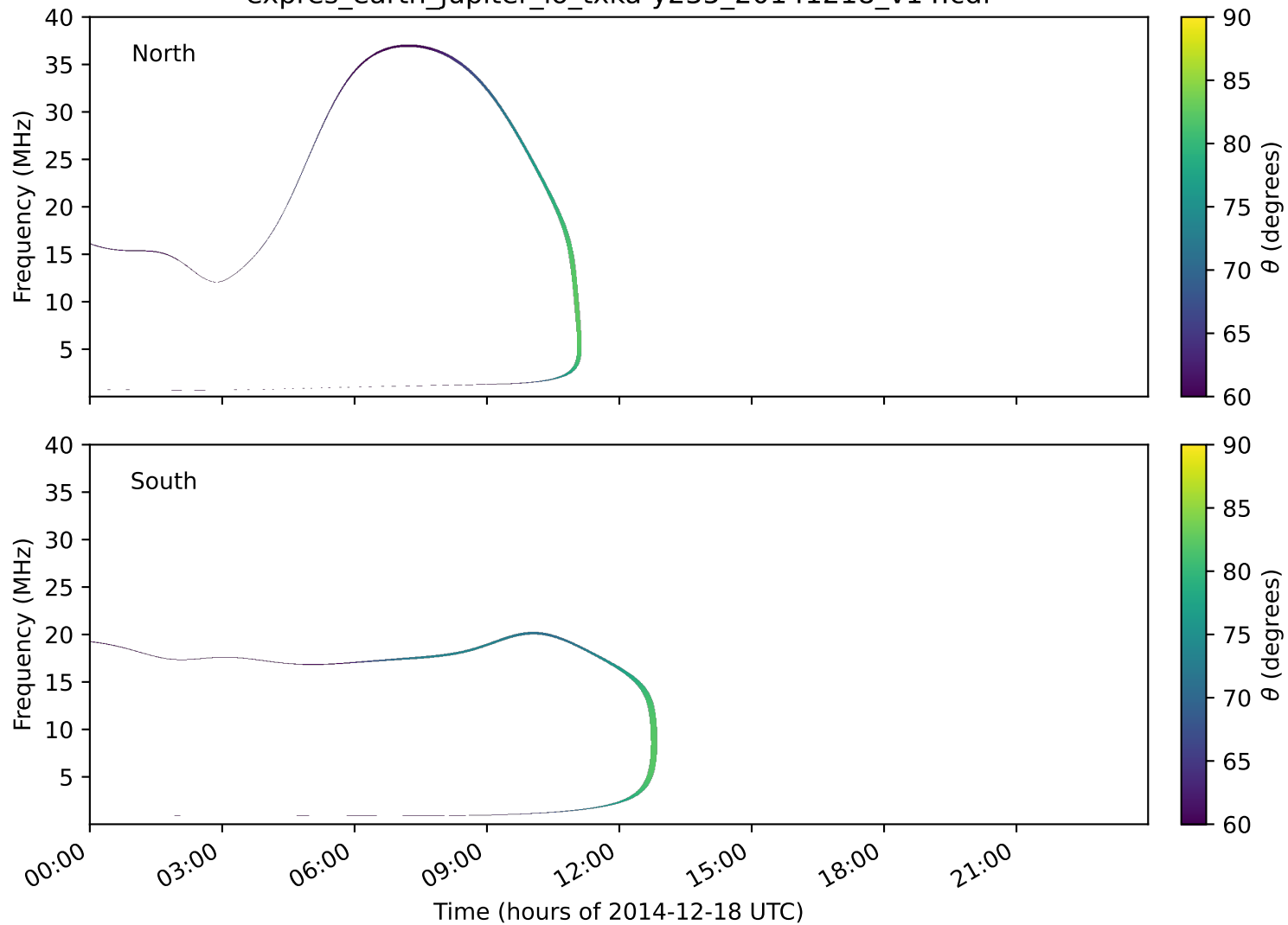
expres_earth_jupiter_io_txka-y235_20141218_v14.cdf
